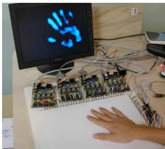
Figure 1: An overview of a tablet size interactive surface based on the SmartSkin sensor.
